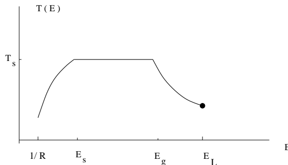
Figure 2. The temperature function in the three-component approximation. Black hole dominance of the density of states at very high energies implies a phase of negative specific heat, starting at E_g \sim 1/g_s^2 (in string units), corresponding to the nucleation of small black holes of size \ell_s , that subsequently grow as the temperature drops. The Jeans energy E_L \sim L^{d-2}/g_s^2 represents the limit beyond which back-reaction effects cannot be neglected on the scale L at the finite-volume box. We have also included the low-energy cutoff at energies of order 1/L because the standard scaling T \sim E^{1/(d+1)} only applies for energies above the gap of finite-volume excitations.
