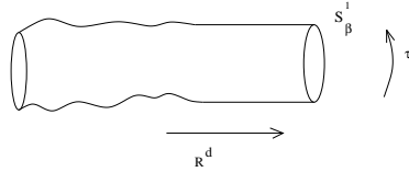
Figure 12. The substitution \beta^2 \rightarrow \beta^2 g_{\tau\tau} has the effect of including local temperature fluctuations on X_\beta .
