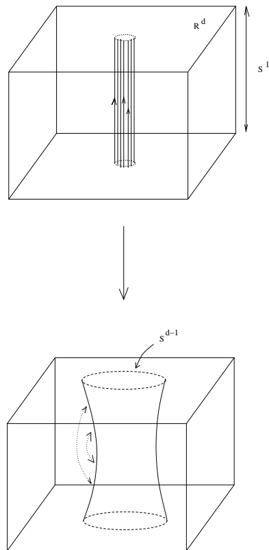
Figure 16. The bottom picture is a local rendering of the basic flop responsible for the Hagedorn transition: \mathbf{R}^d \times \mathbf{S}^1 \longrightarrow \mathbf{S}^{d-1} \times \mathbf{R}^2 , that represents the condensation of many thermal winding strings (top picture). In these drawings, opposite points in the top and bottom planes are identified, together with points reflected about the plane of symmetry of the throat with \mathbf{S}^{d-1} sections.
