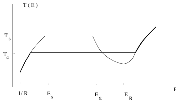
Figure 4. The complete microcanonical temperature function for thermal AdS spaces, in the four-component approximation. In addition to the gravitons, heavy strings and small black holes, we now include large AdS black holes. When small Schwarzschild black holes grow to size R , at energies E_R \sim N^2/R , their specific heat becomes positive and the temperature can grow without bound with T \sim E^{1/d} , corresponding to the dual CFT in d dimensions. A Maxwell construction (in the thick line) shows that the Hagedorn plateau is only accessible to superheated states. A first-order phase transition at T_c \sim 1/R nucleates very large black holes of mass M \sim N^2 R^3 T_c^4 , directly out of the massless graviton phase.
