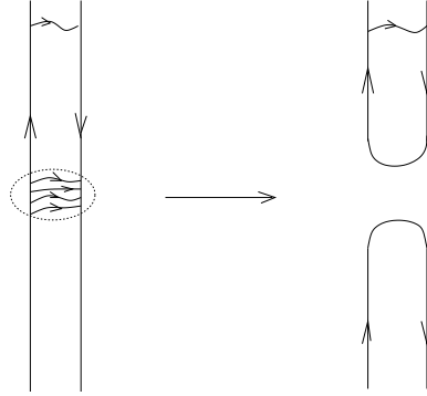
Figure 17. In D-brane annihilation, the condensation of tachyonic strings stretching between the brane and the antibrane can be depicted semiclassically as the reconnection of both Dp -branes. The reconnection generates a throat that is unstable to growth; this throat is nothing but the original stretched string in the “BIon” picture of Ref. [41], in which the string is locally homeomorphic to \mathbf{R} \times \mathbf{S}^{p-1} .
