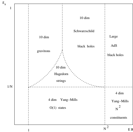
Figure 3. The phase diagram of quantum gravity in \text{AdS}_5 \times \text{S}^5 with N units of Ramond-Ramond flux, according to the AdS/CFT correspondence. A ten-dimensional weakly-curved description only arises for R/\ell_s \sim (g_s N)^{1/4} \gg 1 . In this case, the Hagedorn regime is bounded by black hole and massless graviton phases. It only exists for sufficiently weak string coupling, g_s \ll N^{-9/17} . At very weak couplings, g_s < 1/N , one must use four-dimensional descriptions based on the Yang-Mills degrees of freedom, whereas at strong coupling, g_s > 1 , the diagram mirrors itself by the action of S-duality.
