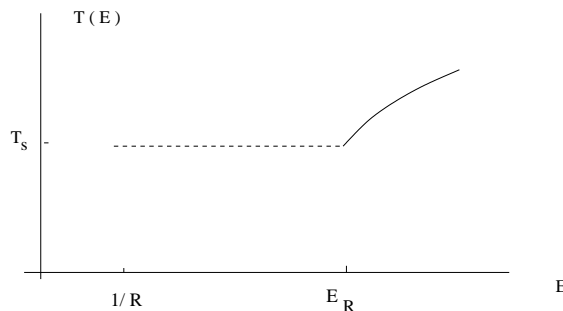
Figure 5. At very weak coupling g_s \sim 1/N , the system matches the perturbative regime of Yang–Mills theory and several hierarchical windows of the system shut down. The ten-dimensional description becomes strongly coupled and standard geometrical intuition breaks down. The string energy E_s that signals the beginning of the Hagedorn plateau becomes of the same order as the finite-size gap of the gauge theory E_{\text{gap}} \sim 1/R , so that the phase of ten-dimensional graviton entropy disappears. The plateau ends at E_R \sim N^2/R , the energy of the phase transition into the Yang–Mills plasma. This threshold coincides with E_g , and the phase of ten-dimensional black holes with negative specific heat also disappears. Instead, the details of the plateau must be worked out in Yang–Mills perturbation theory in the 't Hooft coupling g_s N < 1 .
