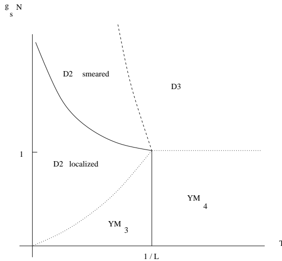
Figure 18. Phase diagram of the D3-brane theory as a function of the 't Hooft coupling g_s N and the temperature, with a compactified direction of length L (c.f. [4]). At weak coupling g_s N < 1 we have the Yang–Mills gas descriptions in four or three dimensions, with the standard threshold for finite size effects at LT \sim 1 . At strong coupling, g_s N > 1 we have the AdS dual description given by the black D3-brane metric at high temperatures. At lower temperatures we have a smooth transition to the smeared black D2-brane metric and then a topological transition to the localized black D2-brane metric. The dotted lines denote correspondence lines between perturbative Yang–Mills descriptions and supergravity descriptions, whereas full lines denote thresholds for finite-size effects on the thermodynamic functions. The localization transition is of first order in the supergravity approximation. The thermodynamic functions calculated in the classical gravity approximation do not change across the T-duality transition (dashed line). The supergravity backgrounds to the left of the T-duality transition are dominated by modes that are interpreted as light winding modes from the point of view of the original D3-brane metric. More general phase diagrams, including effects of large- N nonlinearities appear in [48].
