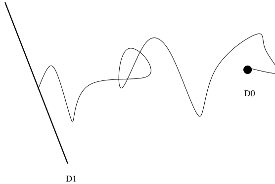
Figure 11. The random configurations of a long string in space are identified with the random paths of of an Euclidean field \chi . Here we show a long open string between D1 and D0 branes or, equivalently, a contribution to the propagator of the thermal scalar.
