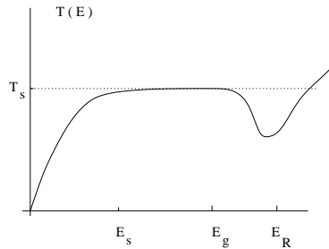
Figure 6. The fine structure of a weakly metastable Hagedorn plateau. The Hagedorn temperature T_s is strictly limiting in this region and the specific heat on the approximate plateau is large and positive, becoming locally unstable for E > E_g . Finite-size effects imply this type of behavior for an ideal gas of closed strings.
