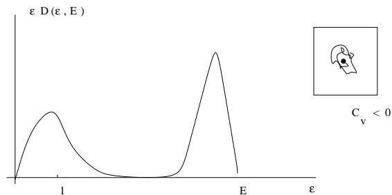
Figure 8. Single-string energy distribution for a total energy E , in systems where the random walks are well-contained and with large co-dimension. The first peak corresponds to the energy in massless modes. The area below it represents the energy deposited in these modes, of order \rho_s V . The second peak corresponds to a single long string that captures E - \rho_s V of the energy. This situation corresponds to an unstable Hagedorn phase, as in figure 7.
