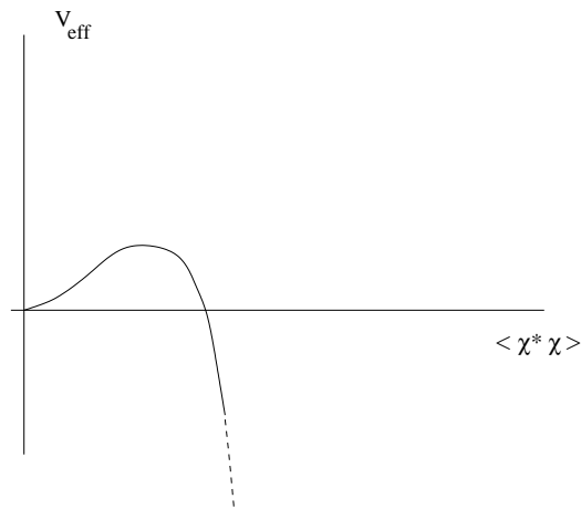
Figure 13. The qualitative form of the thermal scalar potential for \beta > \beta_s .
