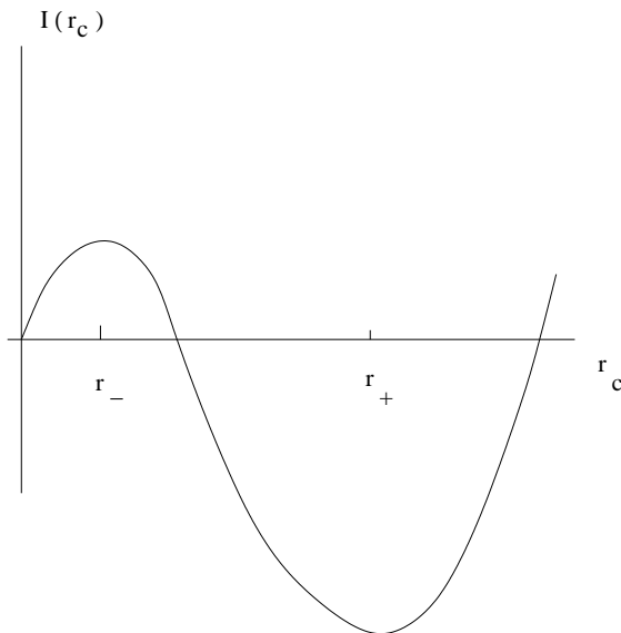
Figure 15. The Euclidean action of off-shell black holes with varying mass and fixed AdS temperature.
