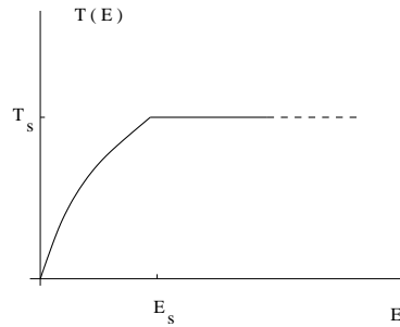
Figure 1. The microcanonical temperature function T(E) = (\partial S/\partial E)^{-1} for a string gas in the two-component approximation. For energies 0 < E < E_s below the string-scale threshold, with E_s = \rho_s V , and \rho_s = O(1) in string units, the temperature grows as T \sim E^{1/(d+1)} , dominated by the massless modes. It gets saturated at T \approx T_s by the highly excited strings. The dotted line represents the sensitivity to small interaction effects that can perturb the Hagedorn plateau either way, into a regime of positive specific heat (with dT(E)/dE > 0 ) or a negative one.
