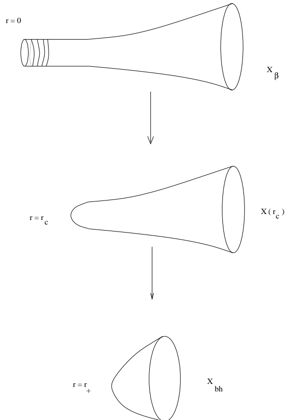
Figure 14. A cartoon of the flow between the original thermal AdS space, with condensing winding modes in the cylinder region r \ll R , and the final Euclidean AdS black hole, which does not support winding modes. A set of interpolating metrics can be interpreted physically as off-shell black holes (c.f. [20, 21]).
