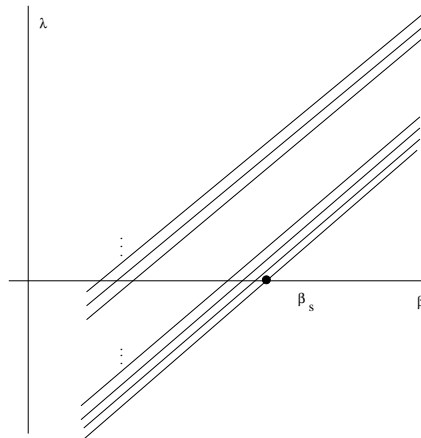
Figure 10. The eigenvalue spectrum of the operator -\nabla^2 + m_{\text{eff}}^2(\beta) in the vicinity of \beta \approx \beta_s . As \beta decreases, there is a lowest eigenvalue that vanishes at \beta = \beta_s . For a finite box of unit size in string units, the eigenvalue spacing is of O(1) and subleading singularities appear below \beta_s separated by O(1) intervals. For a finite box of size L \gg \ell_s , there are associated bands of momentum modes with spacing of order 1/L^2 . In the limit L \rightarrow \infty the bands become quasicontinuous.
