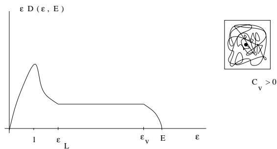
Figure 9. Single-string energy distribution for systems with a very “dense packing” of random walks in the allowed volume. The initial peak of the massless modes decays to a plateau that starts at \varepsilon = \varepsilon_L \sim L^2 , the energy of volume-saturating random walks. The plateau continues up to energies \varepsilon_v \sim E - \rho_s V . This situation corresponds to a locally stable Hagedorn phase, as in figure 6.
