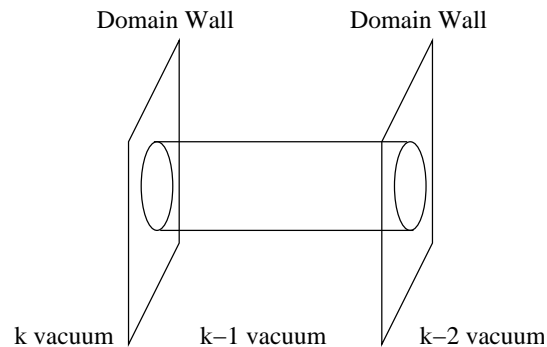
Figure 7. The annulus diagram for the orientifold field theory. The D branes are domain walls. Closed strings are bosonic glueballs and open strings are UV degrees of freedom.
