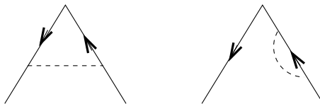
Figure 14. The one-loop anomalous dimension of the bifermion operator (or the mass term). The solid line depicts a fermion, the dashed line a gluon.
