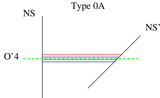
Figure 11. A type-0A brane configuration with an orientifold plane. The field theory on the branes is a U(N) gauge theory with a Dirac fermion in the antisymmetric (symmetric) two-index representation.
