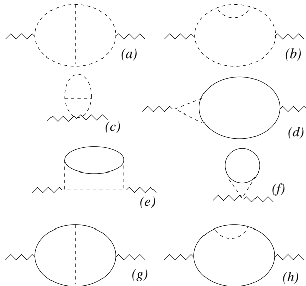
Figure 12. Two-loop contributions to the \beta function. The wavy line is the background (soft) gluon field, the dashed line stands for the quantum gluon field, the solid line for the fermion fields. The fermion contribution is represented by diagrams d through h .
