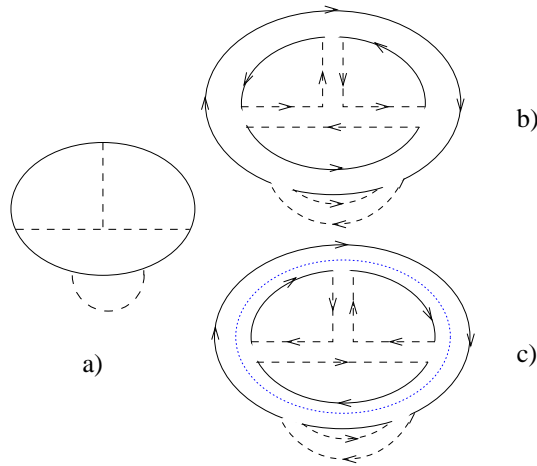
Figure 5. (a) A typical planar contribution to the vacuum energy. (b and c) The same in the 't Hooft notation for (b) \mathcal{N}=1 SYM theory; (c) orientifold daughter.
