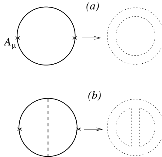
Figure 3. Counting N factors in the correlation function of the axial currents. The 't Hooft diagrams are shown in dashed lines.
