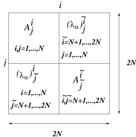
Figure 2. Color decomposition of fields in the Z_2 -orbifold daughter.
