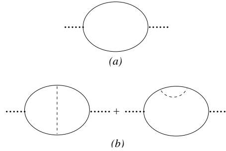
Figure 13. \gamma^* \rightarrow \bar{\psi}\psi \rightarrow \gamma^* in one and two loops. A virtual photon is denoted by the dotted line.
