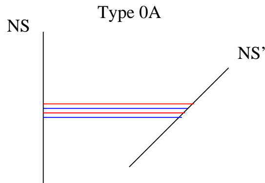
Figure 10. A type-0A brane configuration. The field theory on the branes is a gauge theory with gauge group U(N) \times U(N) and a bifundamental Dirac fermion (the Z_2 orbifold field theory).
