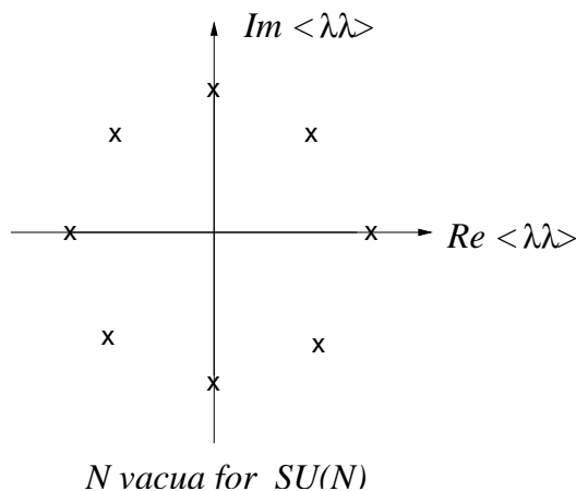
Figure 1. The gluino condensate \langle \lambda\lambda \rangle is the order parameter labeling distinct vacua in supersymmetric gluodynamics. For the SU(N) gauge group there are N discrete degenerate vacua.
