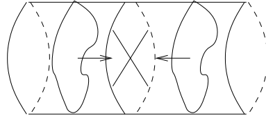
Figure 8. A D-brane, a closed string and their mirrors in the presence of an orientifold plane.
