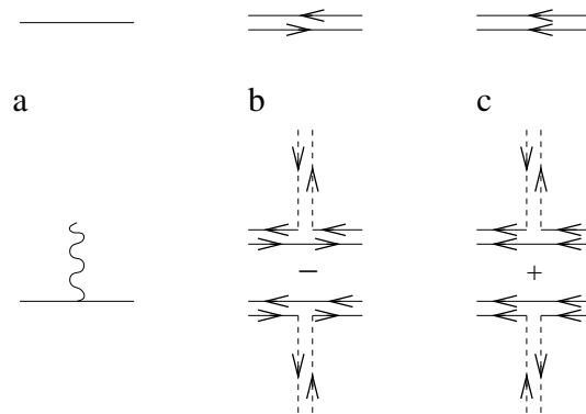
Figure 4. (a) The fermion propagator and the fermion-fermion-gluon vertex. (b) \mathcal{N} = 1 SYM theory. (c) Orientifold daughter.
