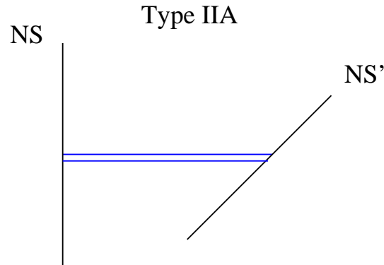
Figure 9. The type-IIA brane configuration. The field theory on the branes is \mathcal{N}=1 SYM theory.
