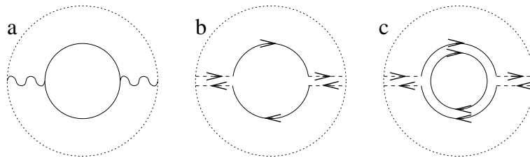
Figure 6. (a.) A typical contribution to the vacuum energy. (b.) The planar contribution in 't Hooft large- N expansion. (c.) The orientifold large- N expansion. The dotted circle represents a sphere so that every line hitting the dotted circle gets connected “on the other side.”
